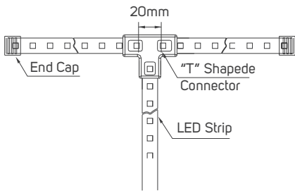
612422 - Middle Connector
