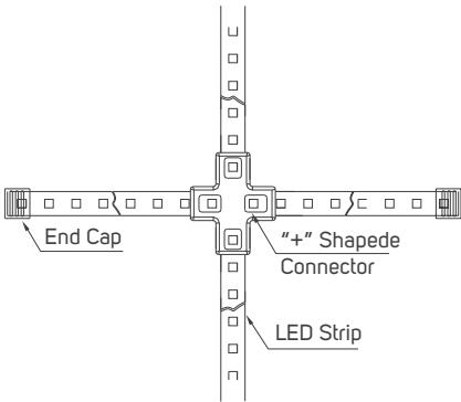
612424 - Middle Connector
