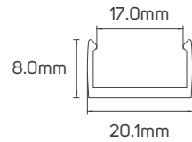
611791 - PVC Profile
