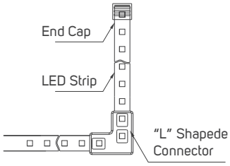
612421 - Middle Connector
