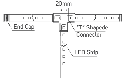
612423- Middle Connector
