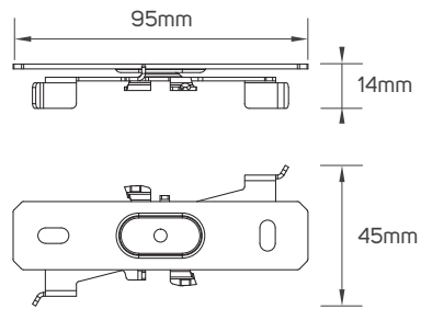
671195 - Connector
