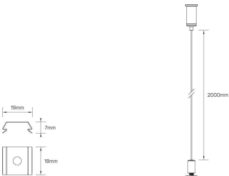
671197 - Connector
