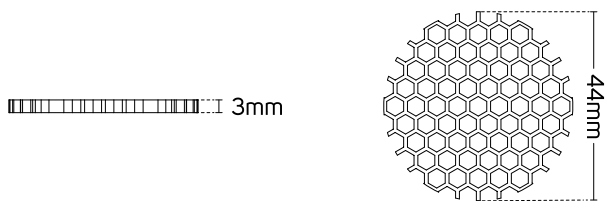
Honeycomb Filter: 5101466
