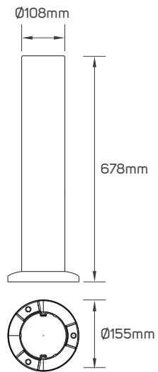
614218 - Tube
