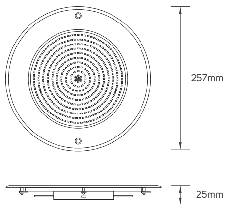
614915 (Cutting Size: D207mm)
