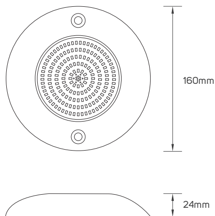
614917(Cutting Size: D20mm)
