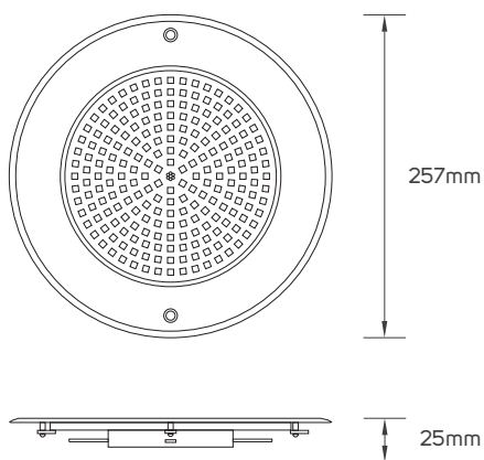
614914 (Cutting Size: D207mm)
