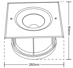
612168 (Cutting Size Ø235)
