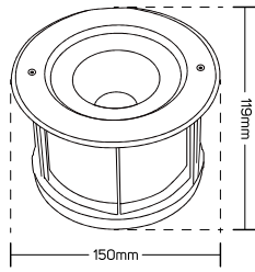
612163 (Cutting Size Ø135)
