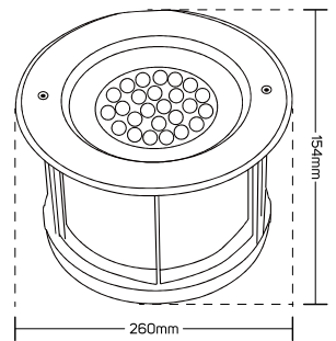
612171 (Cutting Size Ø235)
