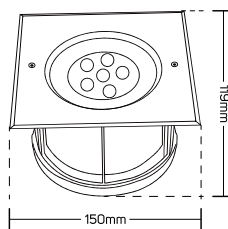
612172 (Cutting Size Ø135)
