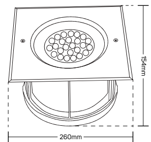
612174 (Cutting Size Ø235)
