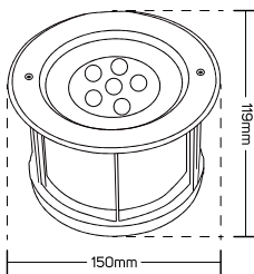
612169 (Cutting Size Ø135)
