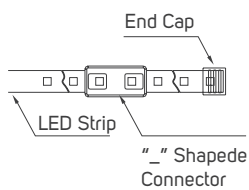
612419 - Middle Connector
