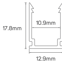
611789 - Aluminum Profile
