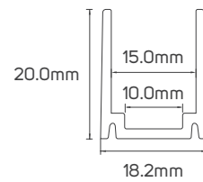
611133 - Aluminum Clip
