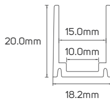
611788 - Aluminum Profile
