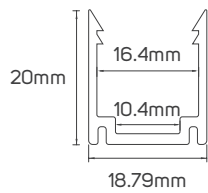
611951 - Aluminum Profile
