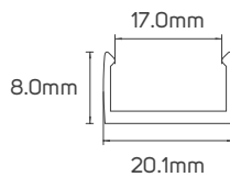
611791 - PVC Profile
