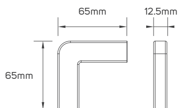
613557 - L Connector
