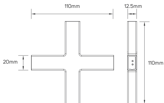
613559 - + Connector
