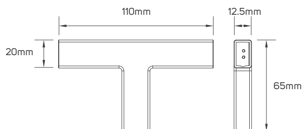
613558 - T Connector
