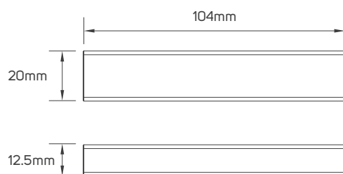
613556 - Connector
