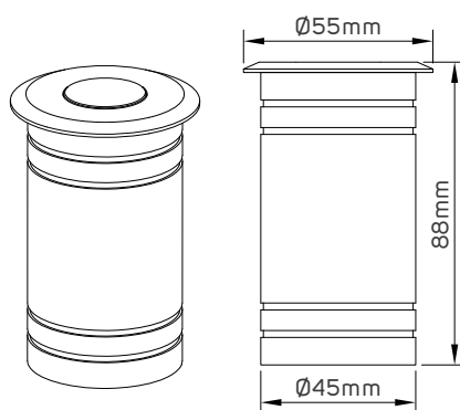
521201, 521306, 521307 (Cutting size Ø45)
