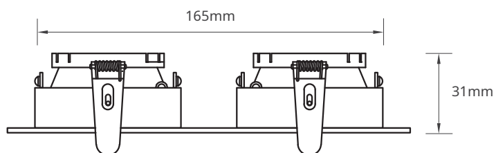
SM241170 - SM241171 (Cutting Size: \varnothing 75\text{mm} )
