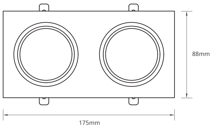
SM241174 - SM241175 (Cutting Size: 16x75mm)
