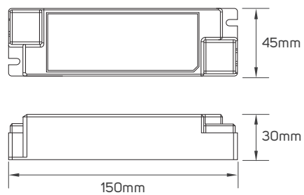
613110 - 613111 - Driver
