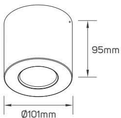
● 613124 - ● 613125 - Surface Mounted Kit
