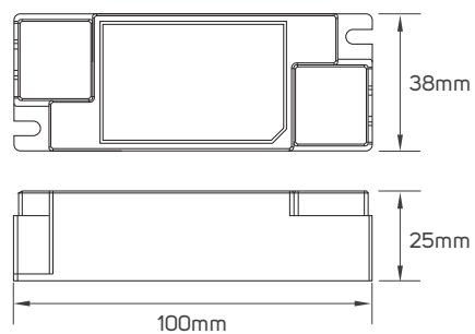
613107 - Driver
