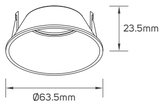
● 613112 - ● 613113 - ● 613114 - Reflector
