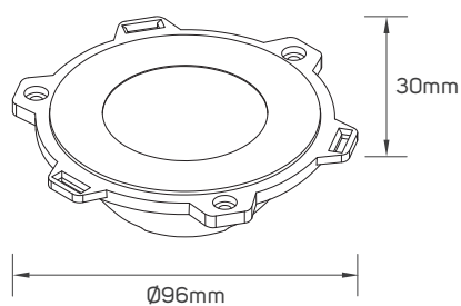
614224 - Lens
